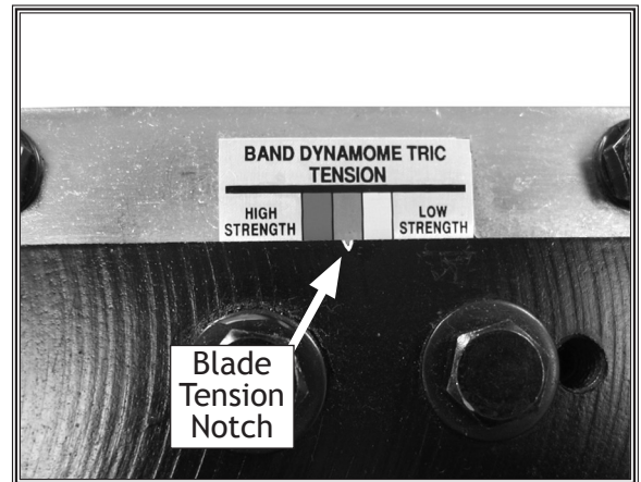
Figure 31. Blade tension scale.
